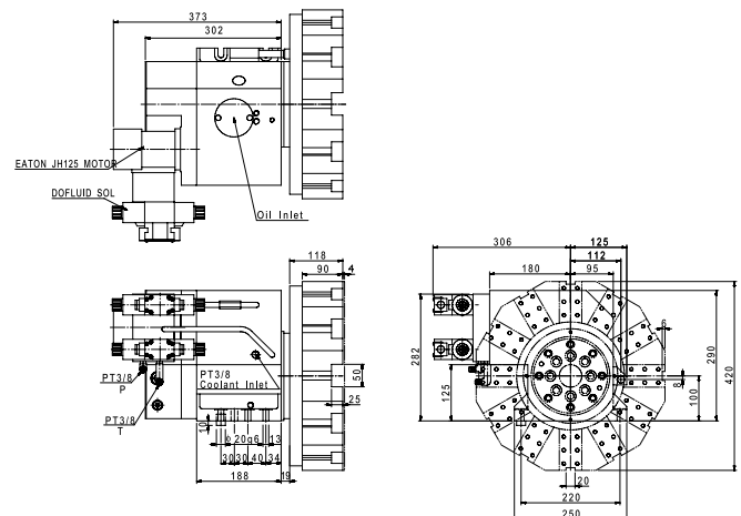
CLT-100-12T
